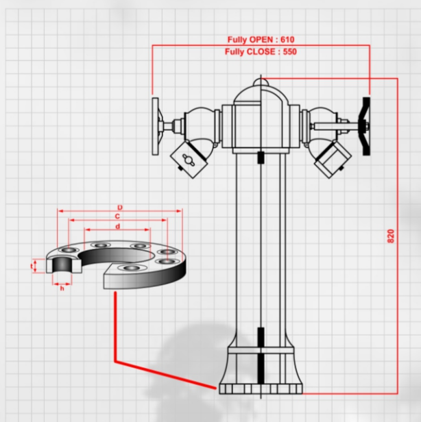
Instantaneous Outlet
